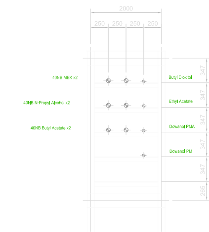
Typical Section 'R-R' Thro' Pipe Bridge
