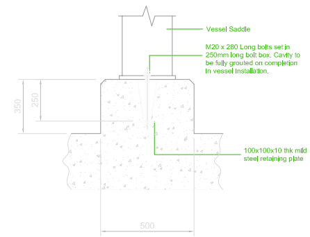
Typical Foundation Bolt Setting
