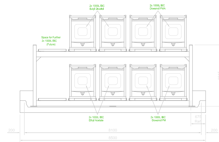
View on Arrow 'A'
