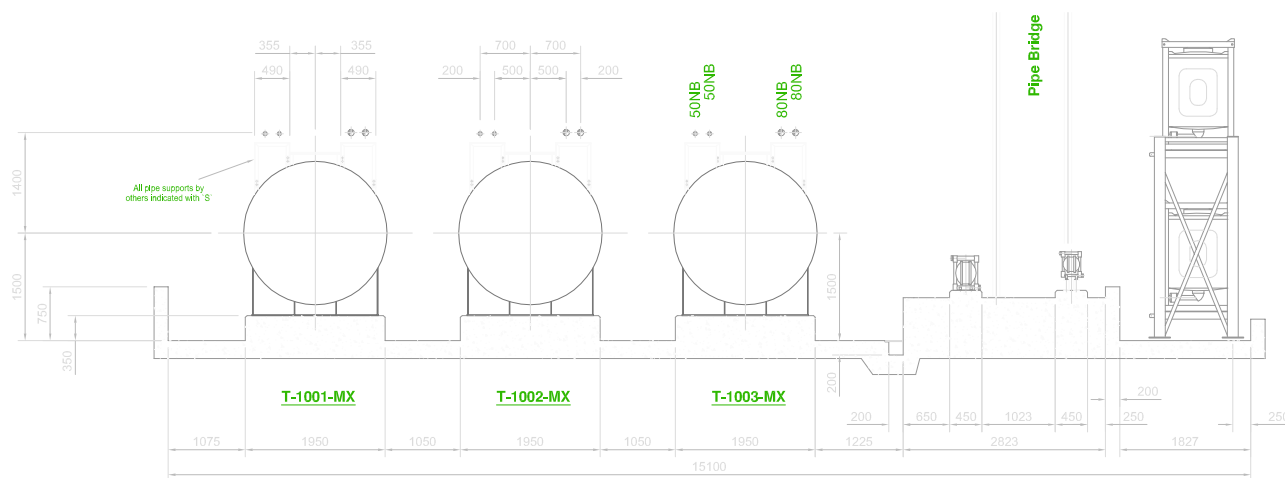
Section 'X-X'
